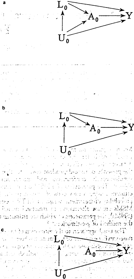
FIGURE 2. Causal graphs for a point exposure A_0 .
