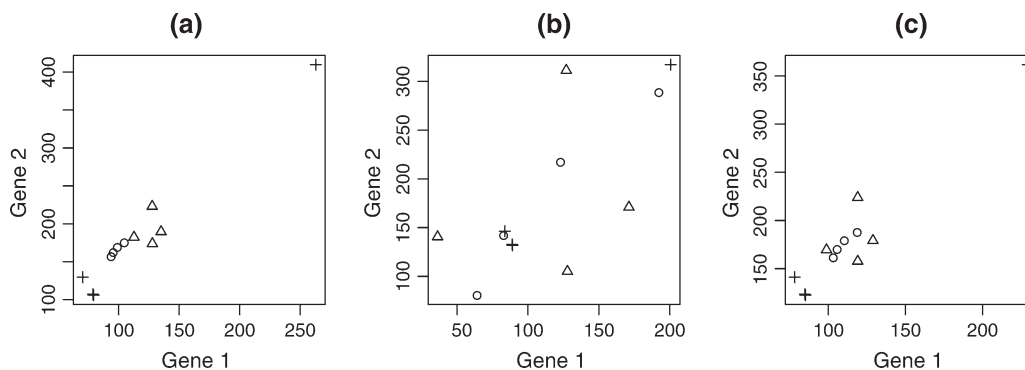
Fig. 4. Plots (a)–(c) illustrate the robustness of the EB adjustments compared to the L/S adjustments. The symbols signify batch membership. Data in (a) are unadjusted expression values for two genes from data set 1; (b) are the L/S-adjusted data. Note that the locations and scales of the batches in (b) have been over adjusted because of outliers in the unadjusted data, and that these outliers disappear in the L/S data; (c) are the EB-adjusted data. The outliers remain in these data and the batch with outliers is barely adjusted. The batches without outliers are adjusted correctly in the EB data.
